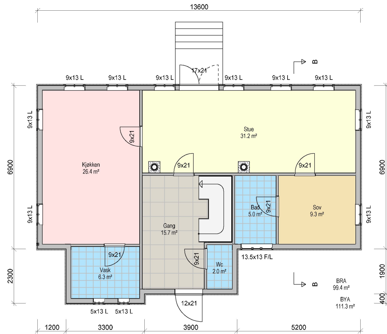
Plan 1 etg
