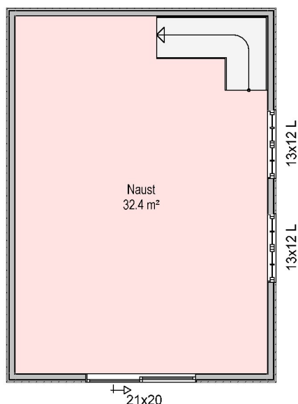
Plan 1 etg
