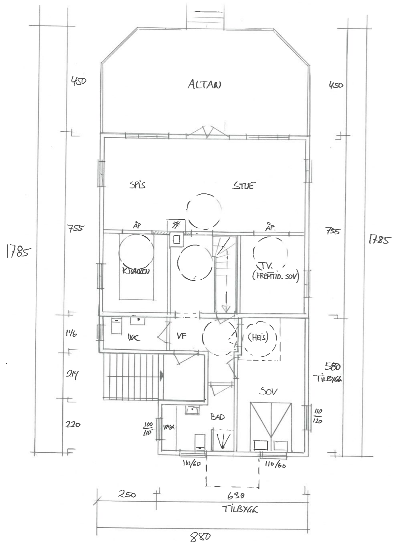
HOVED PLAN
