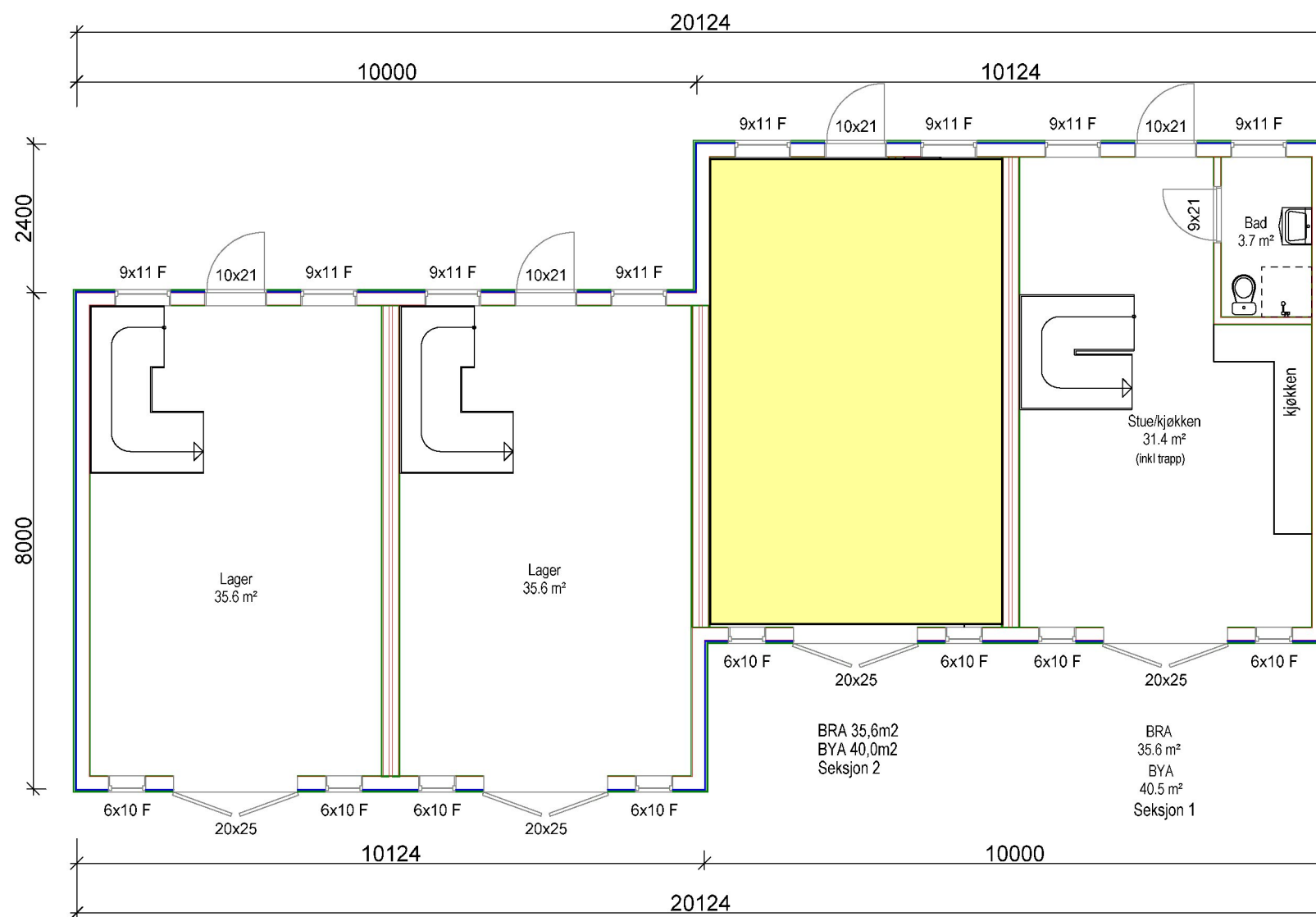
Plan 1 etg
