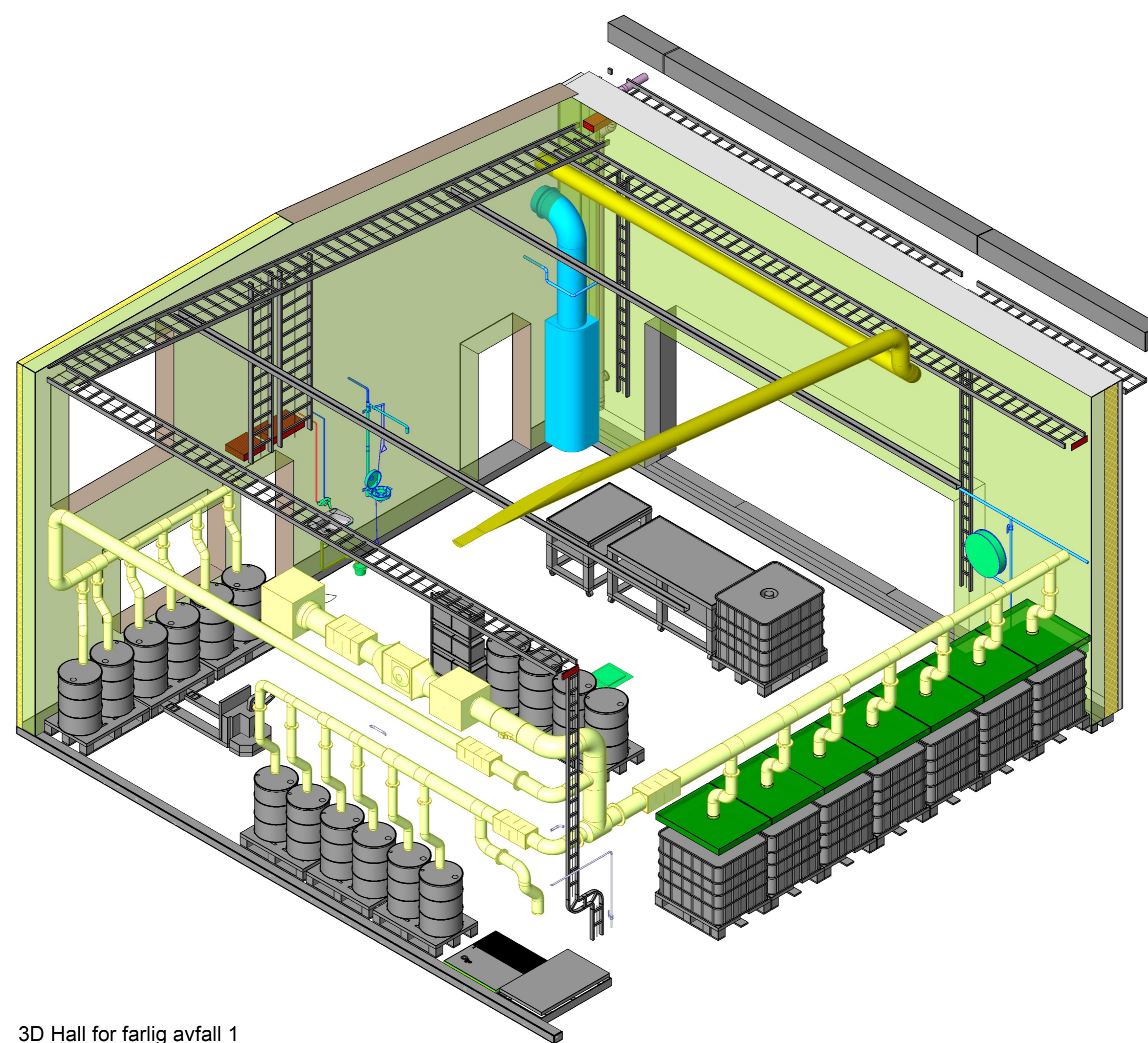
4 3D Hall for farlig avfall 1
