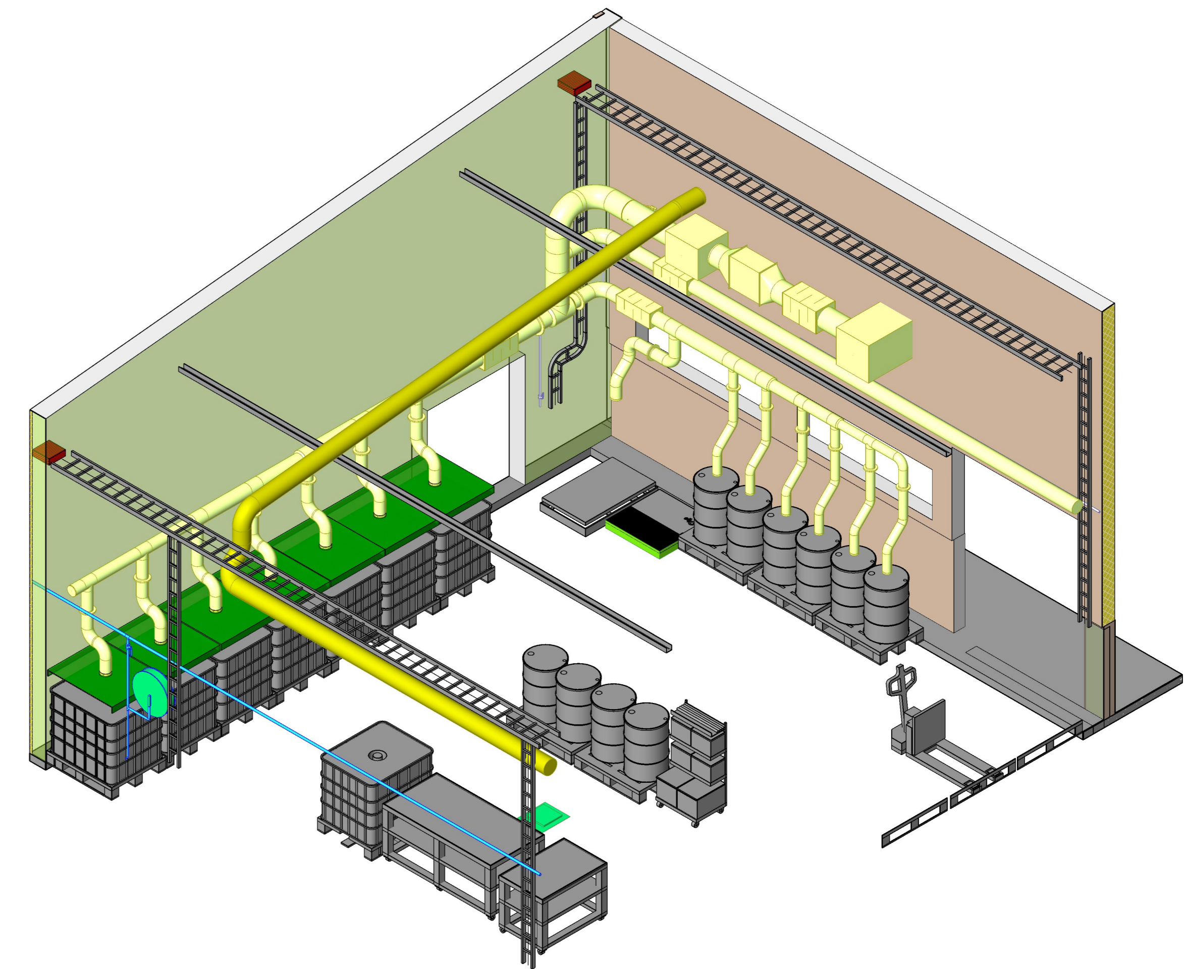
6 3D Hall for farlig avfall 2
