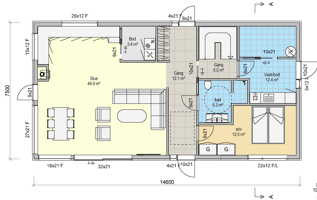
Plan 1 etg
