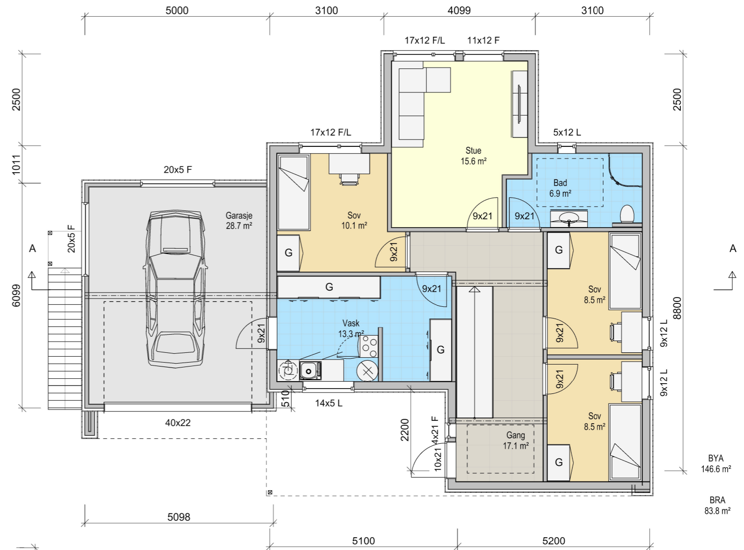
Plan 1 etg
