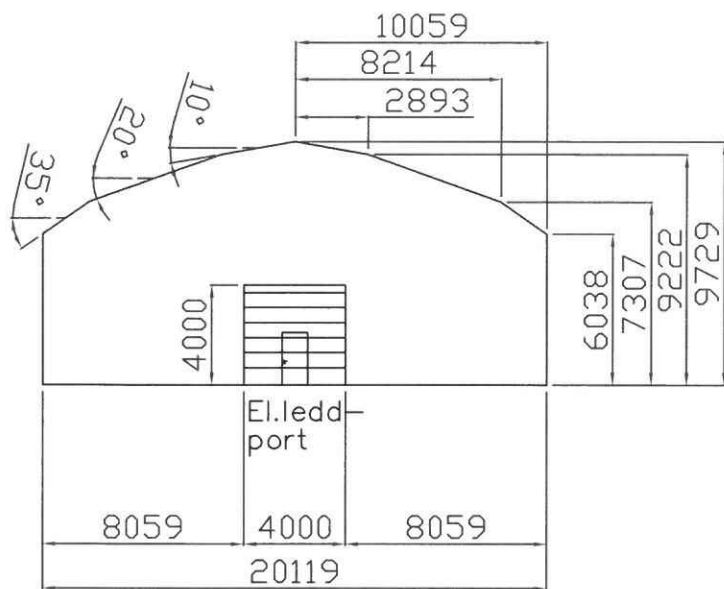
Gavl 1
